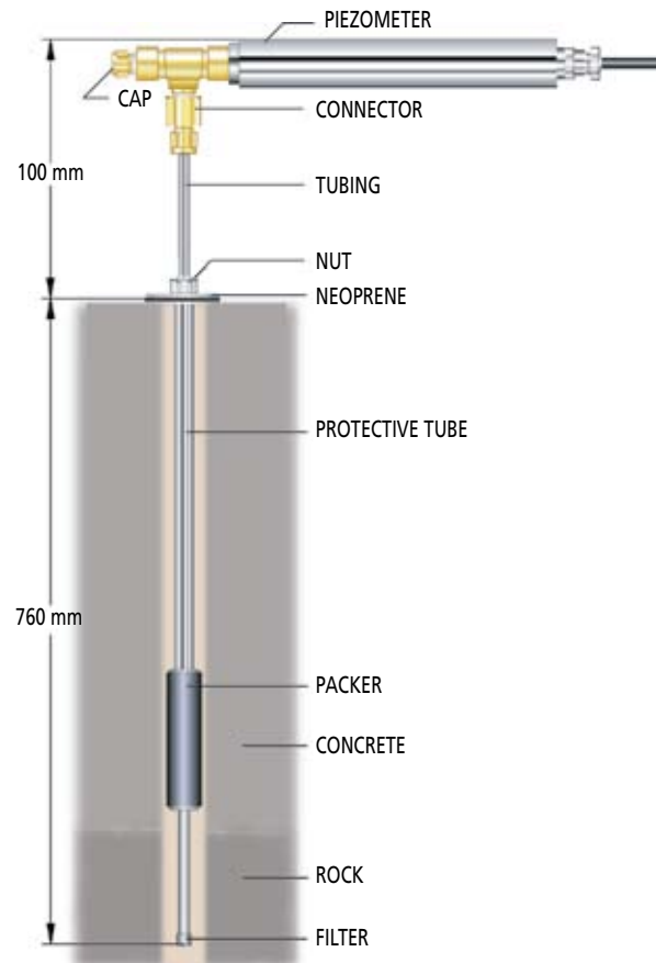
MOD-2A Typical dimensions and installation
