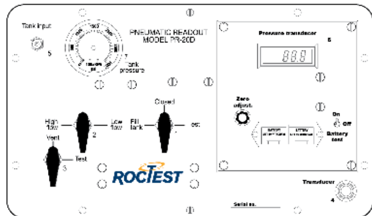
PR-20D Control Panel
